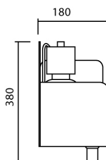
MODEL : MBM-101 (mm.)
