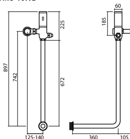
MODEL : MU-107/L (mm.)
